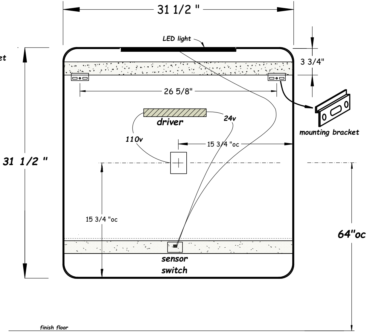
Rear View
